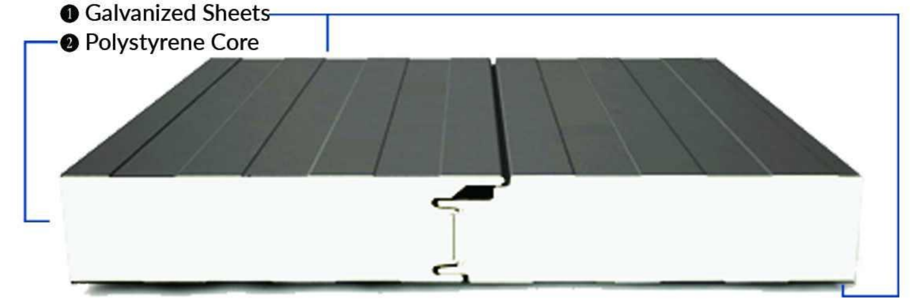
Polystyrene Insulated Sandwich Panels For Walls
